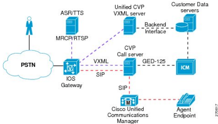
Figure 2: Comprehensive Functional Deployment Model
